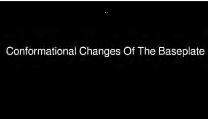
Bacteriophage T4 baseplate conformational change
